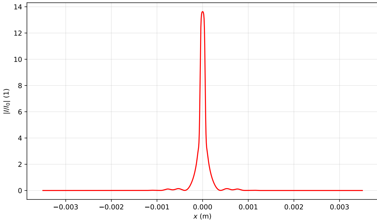
Intensity profile I(x, y = 0, z = 0.716)/I_0 , P_{in}=8.5P_{cr} , artificial time
